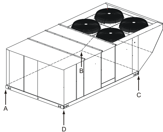
XP240 Unit 4 Point Load Weight
